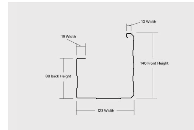
FASCIA GUTTER (VIC)
