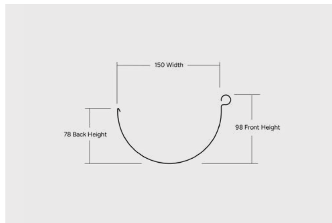
150 HALF ROUND (VIC, SA, TAS)
