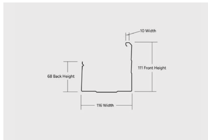
COMPACT GUTTER (QLD)
