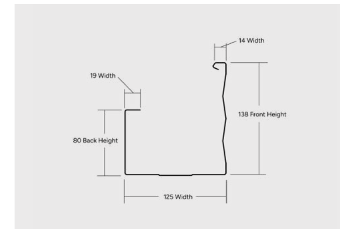
TRILINE® SIFFENED BACK (NSW)
