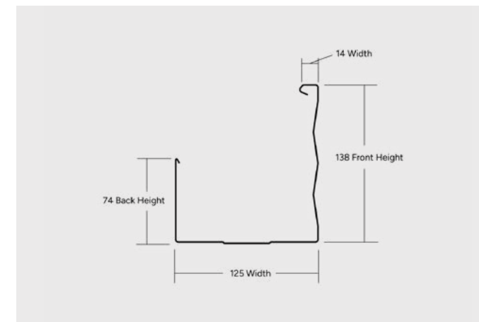
TRILINE® HOOKBACK (NSW)
