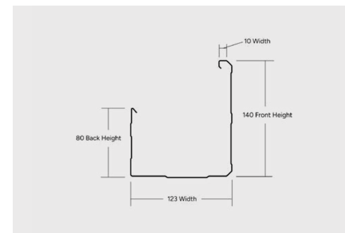
M PATTERN FASCIA GUTTER (QLD, NSW)
