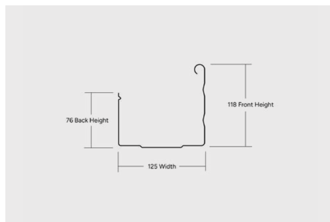
EASIFLOW GUTTER (VIC, TAS)
