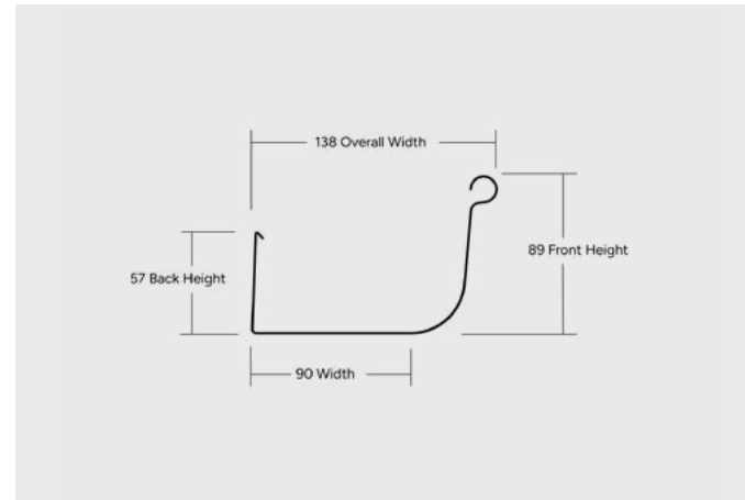
QUAD 115 HI-FRONT (NSW) QUAD 115 (VIC)
