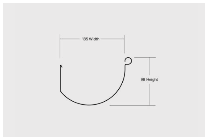
HALF ROUND FLATBACK (VIC, SA, TAS)
