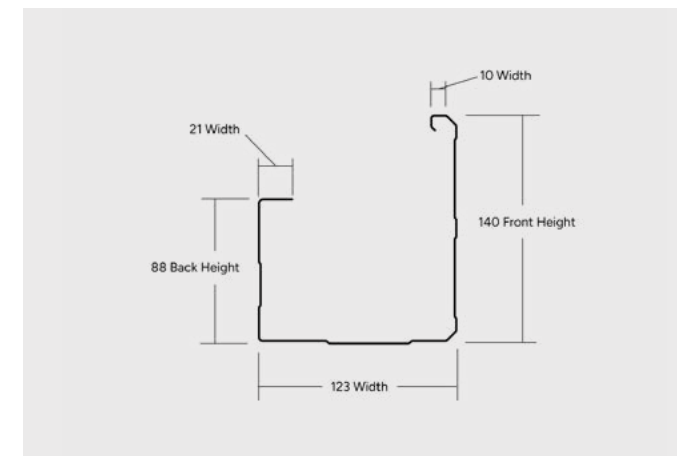
S PATTERN FASCIA GUTTER (QLD, NSW)
